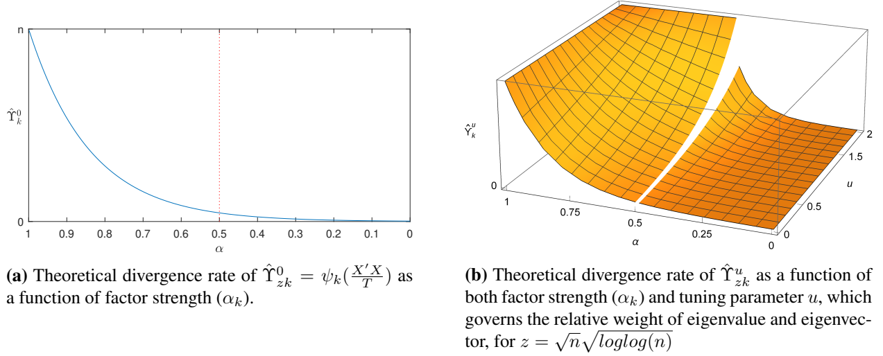
Figure 2: Illustration of theoretical divergence rates for key quantities. Figure created with n = 500 .
