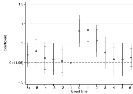
(a) Event-study plot for outcome
